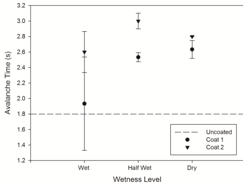
Figure 4-9: Avalanche time of coated pellets at different wetness levels compared to the baseline avalanche time of uncoated glass pellets
